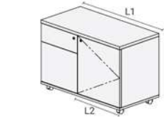
With Door S-A-SR-800_S-A-SR-900L-R / L L1 800 x L2 381 x W 450 x H 600 mm L1 900 x L2 481 x W 450 x H 600 mm
