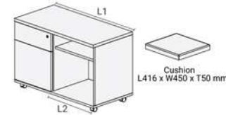
S-A-SR-800_S-A-SR-900L-R / L L1 800 x L2 387 x W 450 x H 600 mm L1 900 x L2 487 x W 450 x H 600 mm
