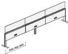
3 Frame Length: 4500 / 4800 / 5400 [mm] Height: 1170 [mm] Thickness: 75 [mm]
