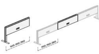
Width: 1500 / 1600 / 1800 [mm] Height: 770 [mm] Thickness: 75 [mm]
