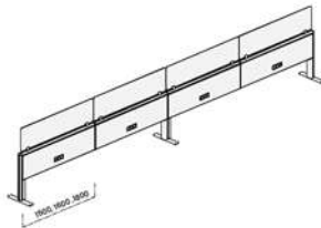
4 Frame Length: 6000 / 6400 / 7200 [mm] Height: 1170 [mm] Thickness: 75 [mm]
