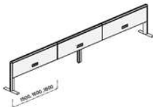
3 Desks Length: 4500 / 4800 / 5400 [mm] Height: 770 [mm] Thickness: 75 [mm]
